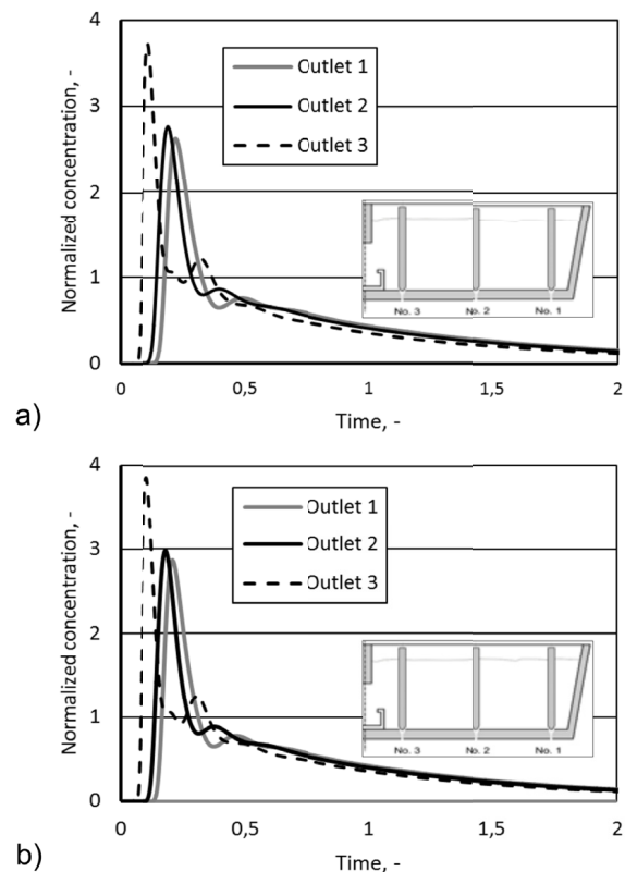
Fig. 7. RTD characteristics of E type: a) 0.98 \text{ m}\cdot\text{s}^{-1} ; b) 1.1 \text{ m}\cdot\text{s}^{-1} [10]
