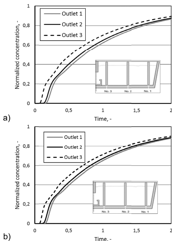
Fig. 6. RTD characteristics of F type: a) 0.98 \text{ m}\cdot\text{s}^{-1} ; b) 1.1 \text{ m}\cdot\text{s}^{-1} [10]
