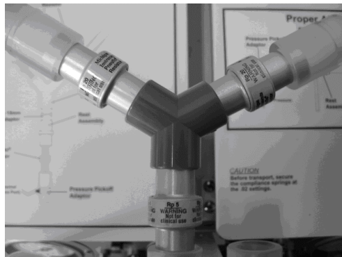
Fig. 4. Adjustable resistive elements modeling the upper airways and bronchial resistance.
