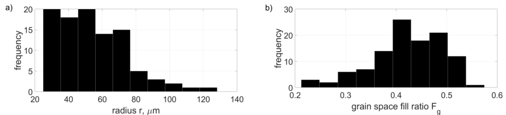
Fig. 8. A histogram of: a) radii r circumscribed on grain tips; b) the coefficient F_g of filling by grains the space on the abrasive tool active surface for h = 20 \mu\text{m} .
