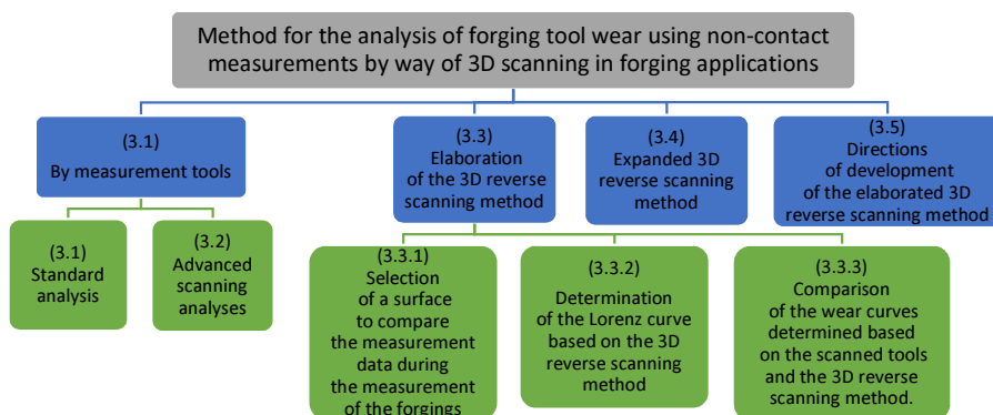
Fig. 3. A block diagram of evaluation of the method of forging tool wear analysis.
