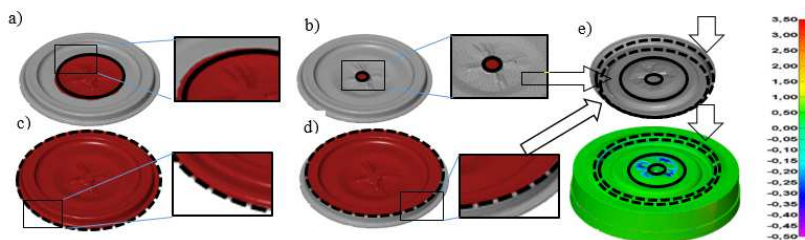
Fig. 19. An example of determining the volume in selected areas: the core volume for area A (a) the total volume for area A (b); the core volume for area B (c); the total volume for area B (d); a schematic diagram of the volume measurement (e).
