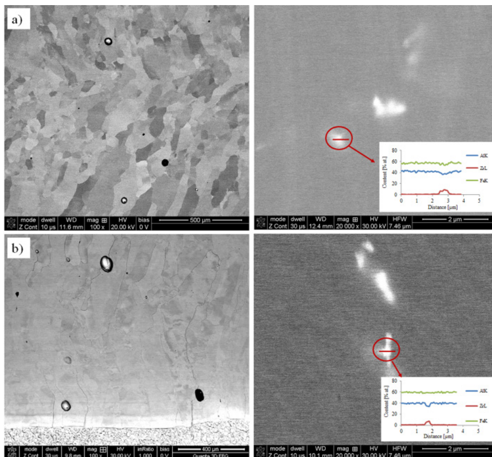
Fig. 4. SEM microphotographs showing microstructural features of a) the FeAl and b) the FeAl with n\text{-Al}_2\text{O}_3 addition samples
