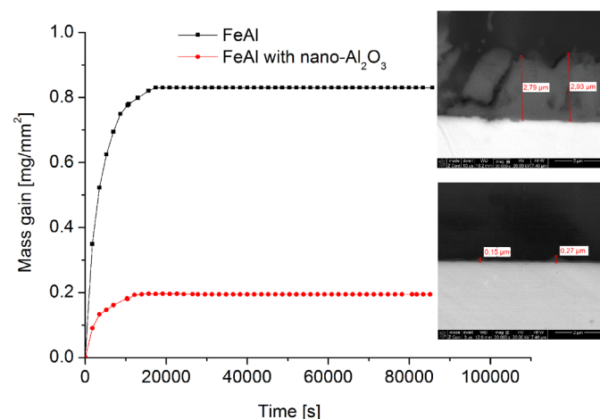
Fig. 9. Mass gain vs. oxidation time plots obtained for the FeAl and FeAl+ n\text{-Al}_2\text{O}_3 samples
