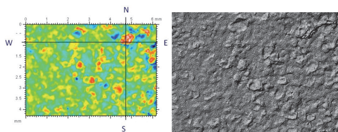
Fig. 3. Geometric shape of the test surface, colour intensity map (left), numeric photograph of the sample surface (right), sand cast alloy
