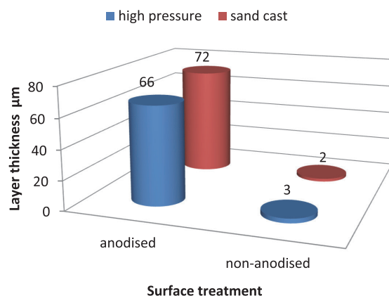
Fig. 1. Comparison of wear resistance of sand cast alloys and high pressure cast alloys
