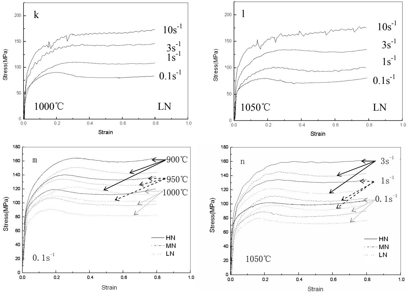
Fig. 1. True stress-strain curves of the experimental steels deformed under various deformation conditions
