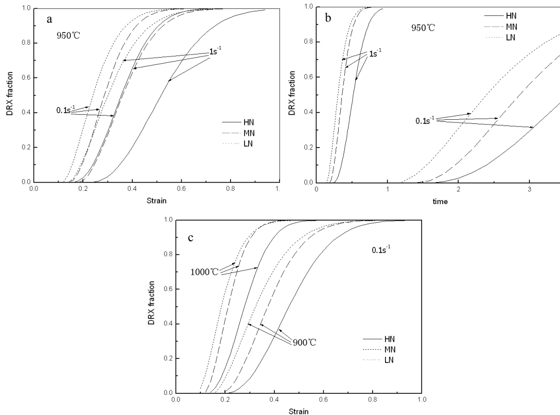
Fig. 5. Relation between DRX volume fractions and (a) strain at 950°C (b) deformation time at 950°C (c) strain at 0.1s^{-1}
