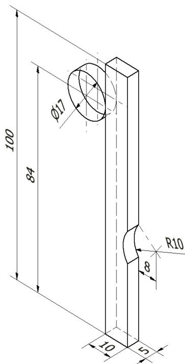
Fig. 2. Dimensions of the sample and the guide roll
