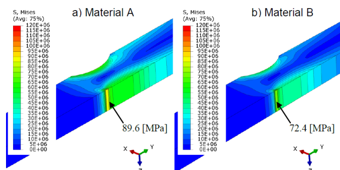
Fig. 4. Stress map according to the Huber-Mises-Hencky theory for the deflection of 0.2 mm
