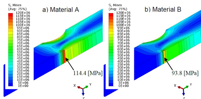
Fig. 5. Stress map according to the Huber-Mises-Hencky theory for the deflection of 0.3 mm
