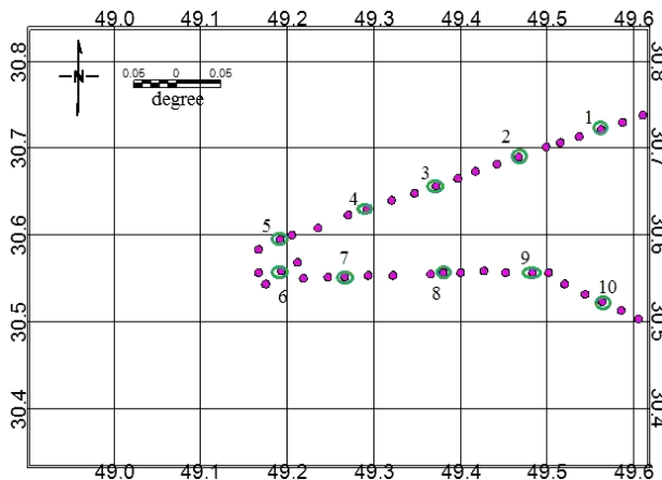
Fig. 7. Enlarged the under study area in Khuzestan as shown in Fig. 4. Purple points refer to GPS/Levelling benchmark while the points circled in green are the determined ones in order to measure correlation coefficient between Sjöberg method and GPS/Levelling data
