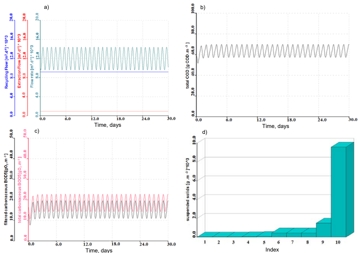
Fig. 5. Simulation results of the transfer of wastewater from M'Daourouch to Sedrata wastewater treatment plant: a) the appropriate mass budget, b) (COD \text{g}\cdot\text{m}^{-3} ) concentration output, c) (BOD \text{g}\cdot\text{m}^{-3} ) concentration output, d) suspended solid fraction in the clarifier; source: own study
