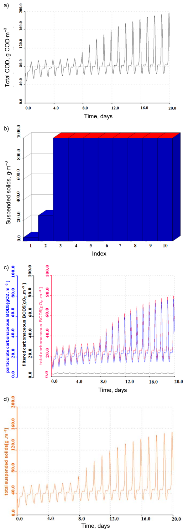
Fig. 8. Effect of the extraction rate on the plant operating performances: a) (COD g·m -3 ) concentration output, b) suspended solid fraction in the clarifier, c) (BOD g·m -3 ) concentration output, d) (total S_s g·m -3 ) concentration output; source: own study
