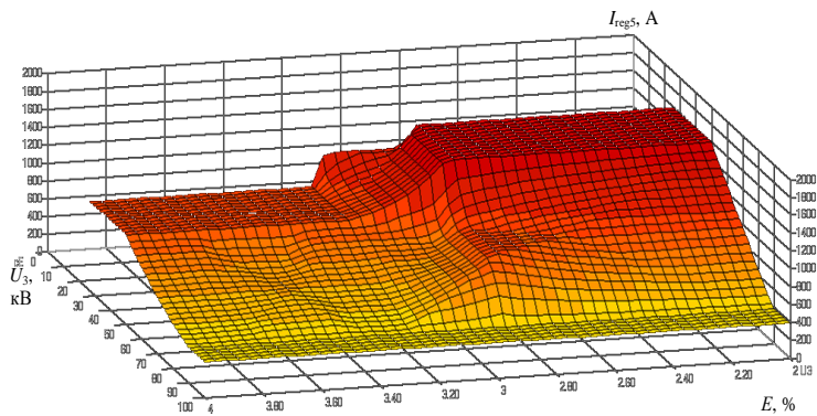
Fig. 6d. Decision-making area for equations I_{reg5} = f(E, U_3)
